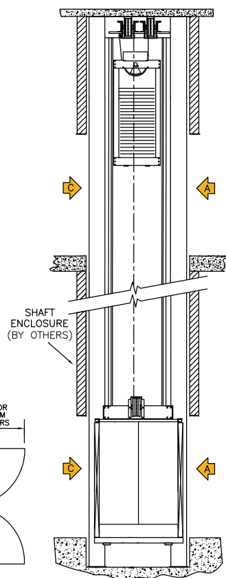
TYPICAL SECTION showing through-car arrangement
