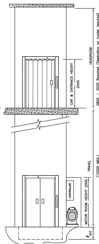
TYPICAL FRONT ELEVATION from "C" face
