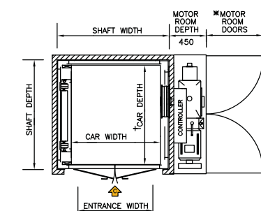
PLAN SECTION showing single entrance arrangement
